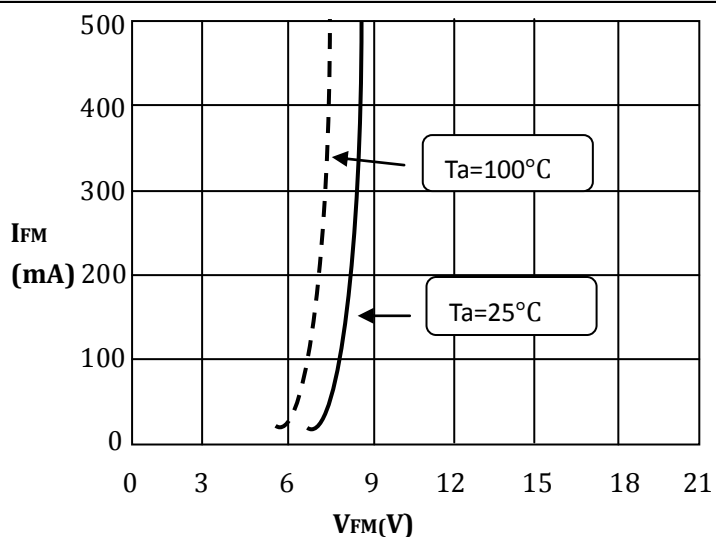
Forward Characteristics
